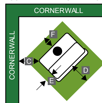
CORNERWALL INSTALLATION
